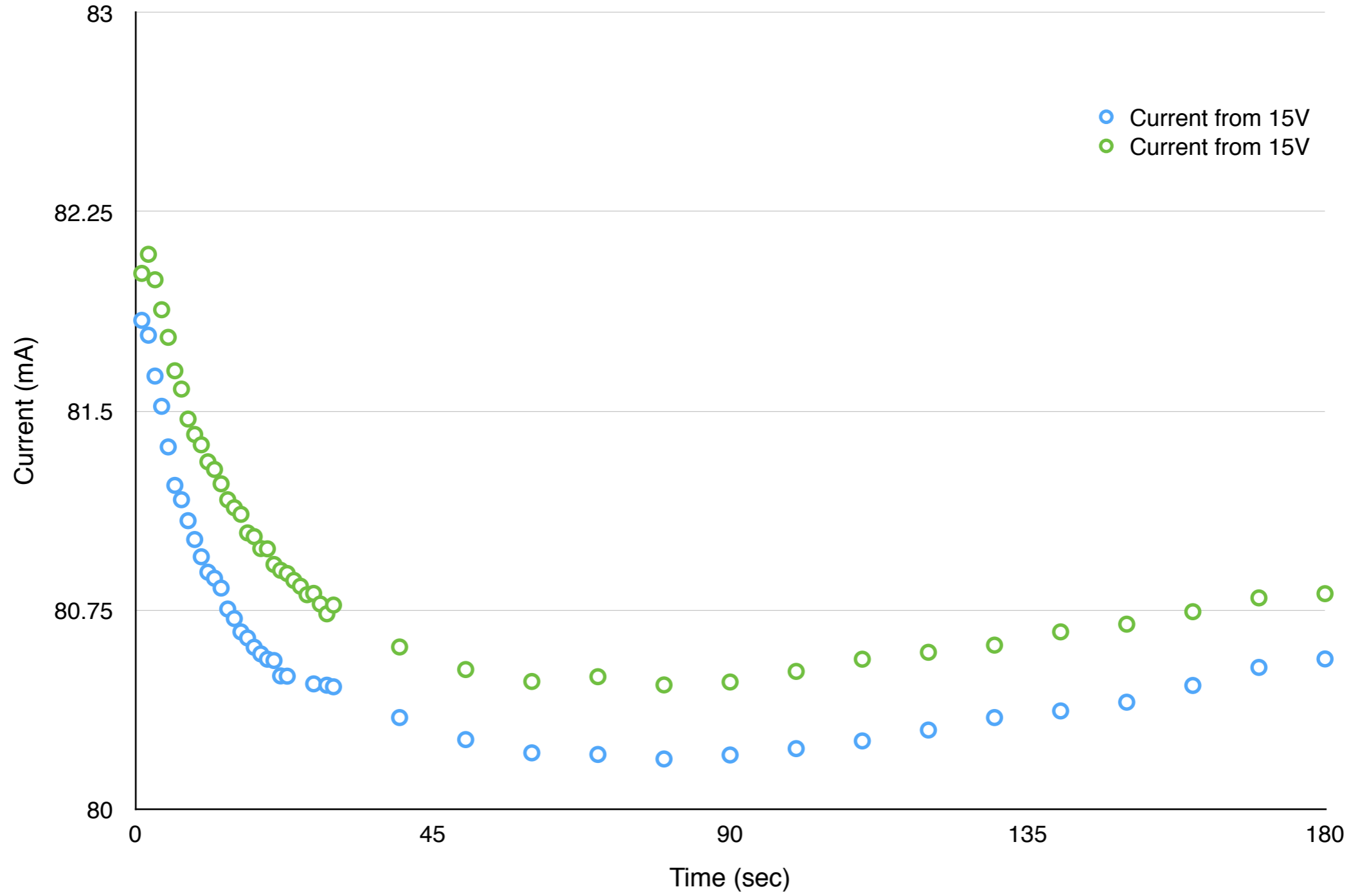
Current vs. Time Active (LWDAQ)
