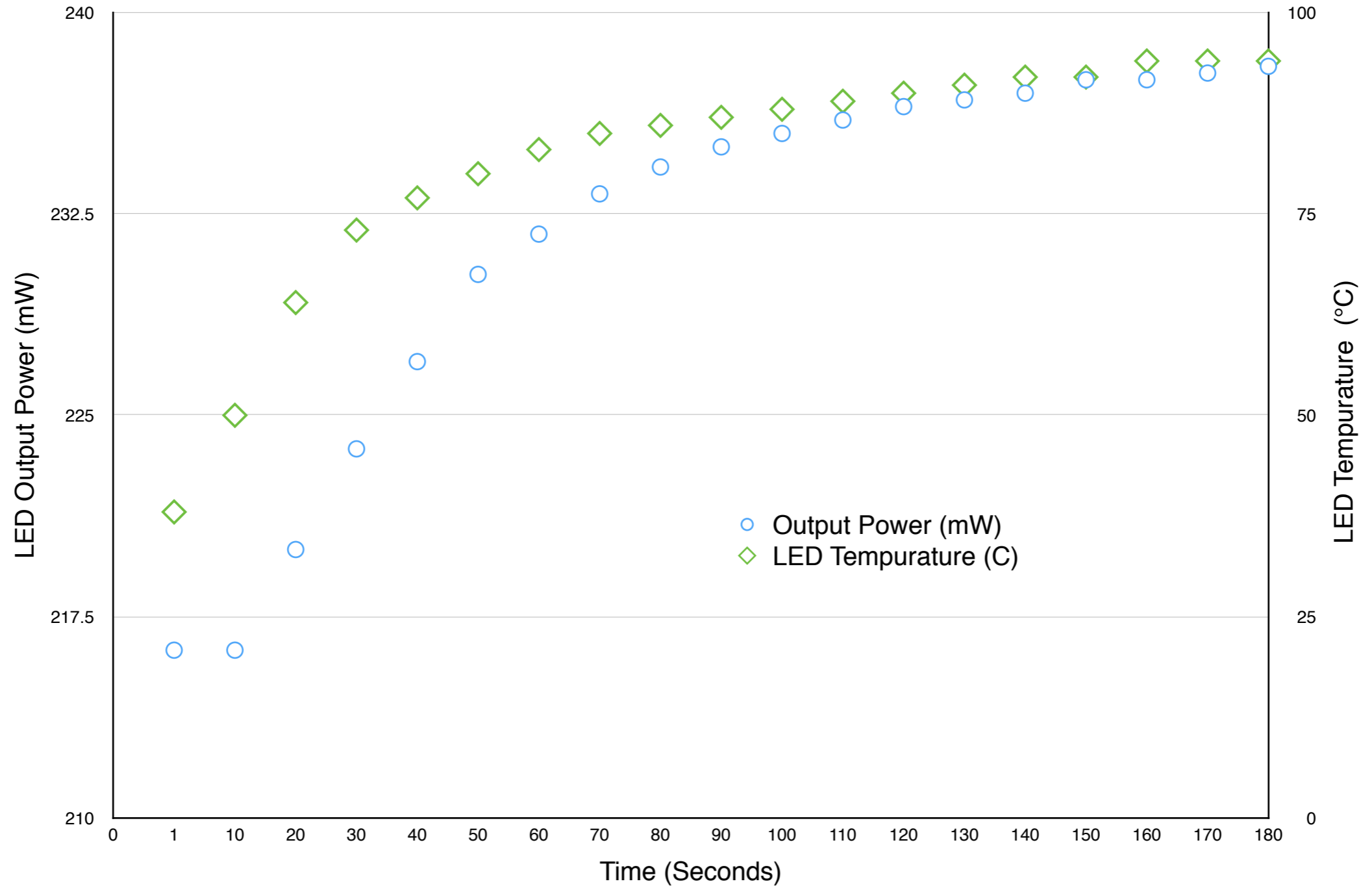
LED Power Output and Temperature vs. Time Active
