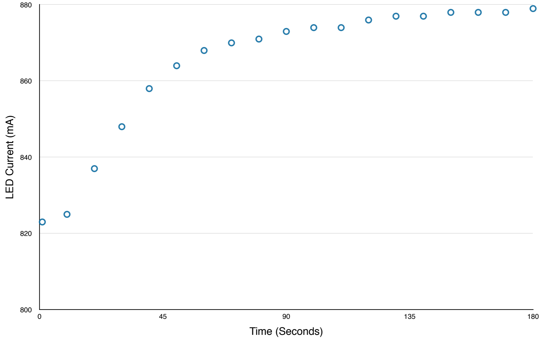
LED Current vs. Time Active
