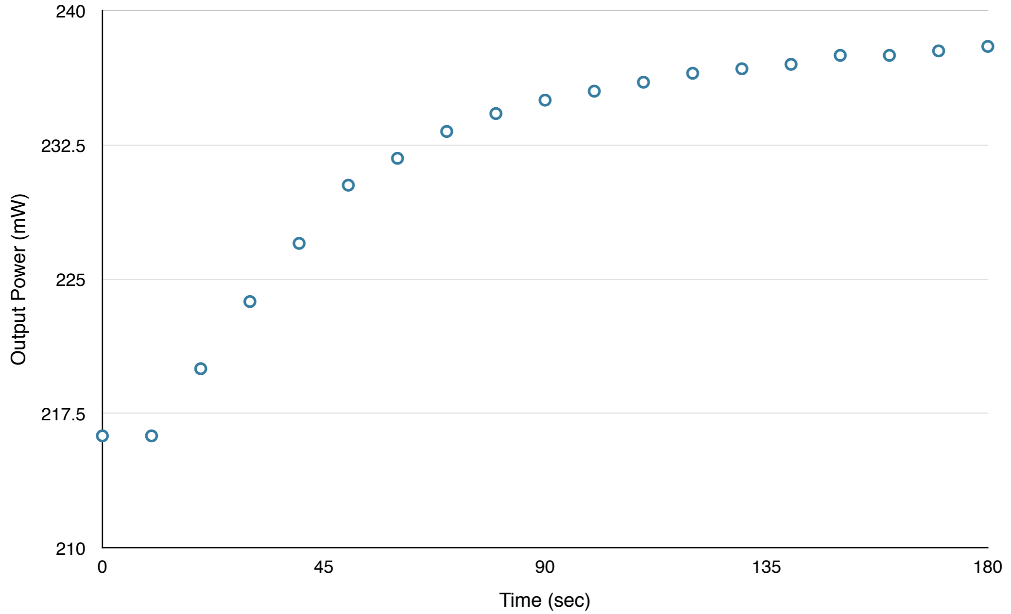
Measured Power Output of LED vs. Time Active
