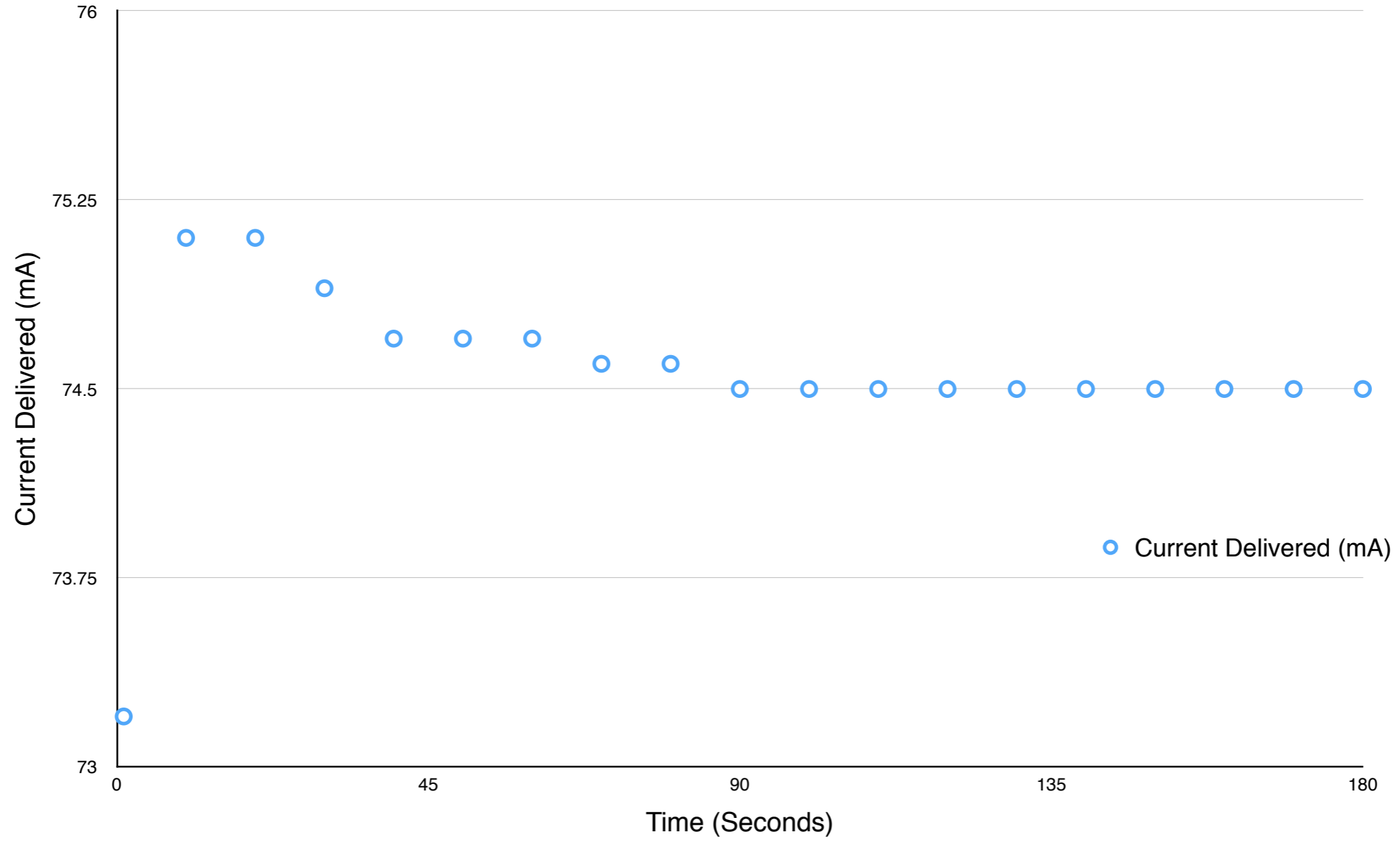
Current from 15V (Through Interface Resistor)
