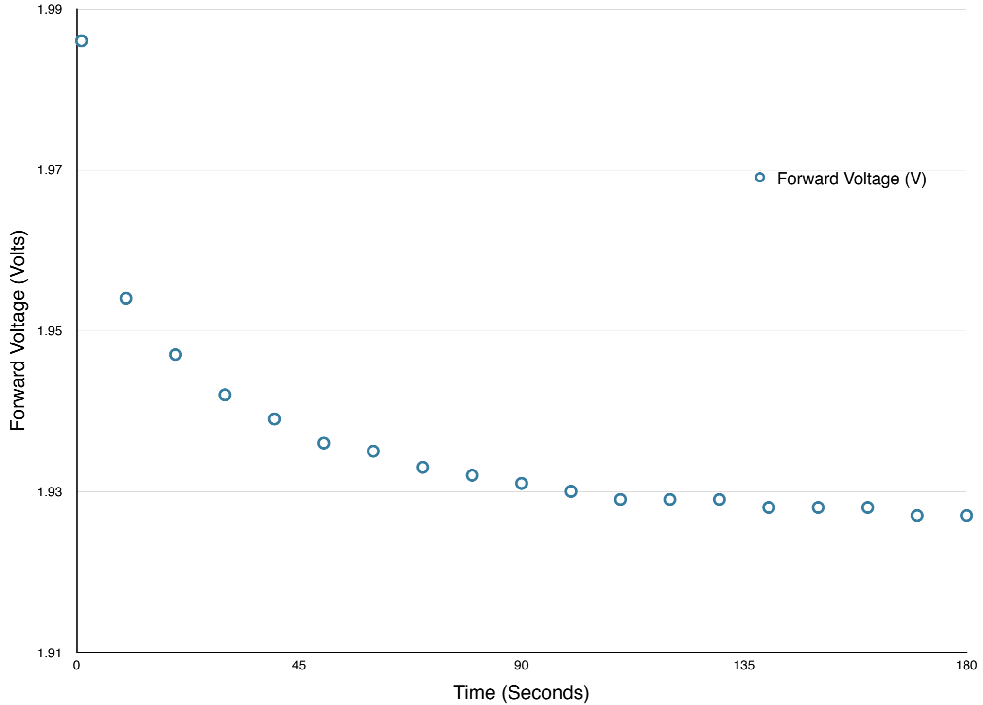
LED Voltage vs. Time
